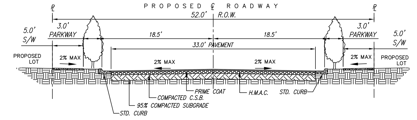
TYPICAL 52' ROW ROAD SECTION (MONTOYA SIERRA DR., MONTOYA ALTO DR., SIERRA BELLO ST., SIERRA ALTO ST.)
