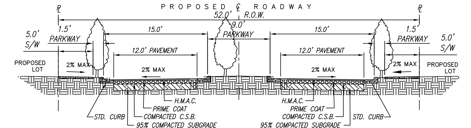
TYPICAL 52' ROW ROAD SECTION (W/ CENTER ISLAND)
