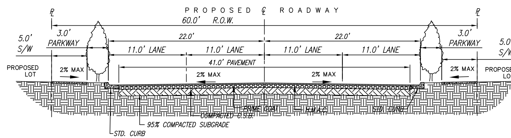
TYPICAL 60' ROW ROAD SECTION (MONTOYA DR.)
