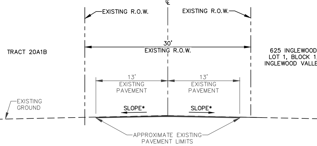
EXISTING INGLEWOOD DRIVE 30' ROW STREET SECTION DETAIL SCALE: 1"=10'
