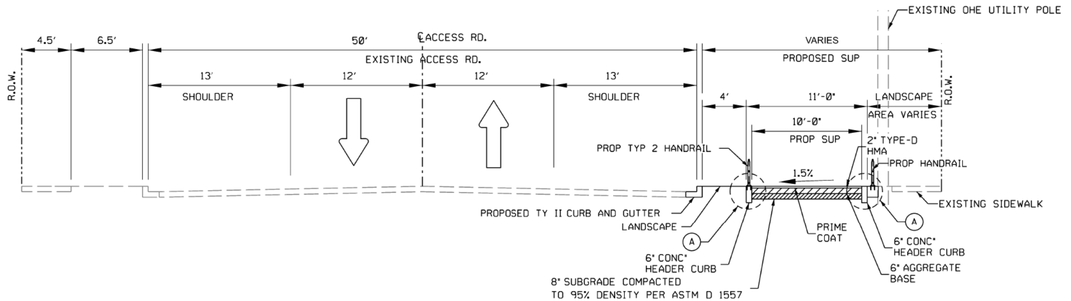
ACCESS ROAD PROPOSED TYPICAL SECTION STA 34+88 TO END
