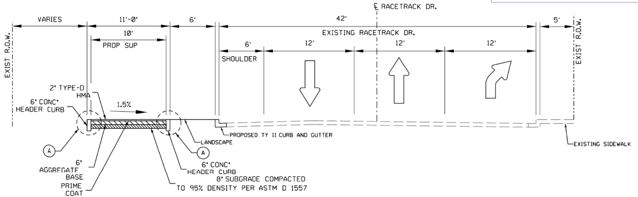
RACETRACK PROPOSED TYPICAL SECTION
