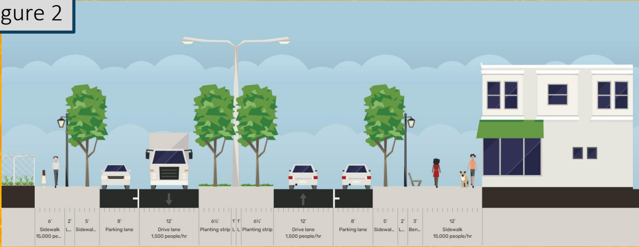
Proposed Cross Section Approaching Montana Ave.
