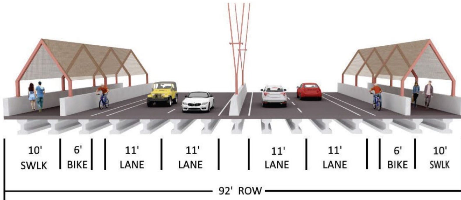
PROPOSED TYPICAL SECTION ON BRIDGE
