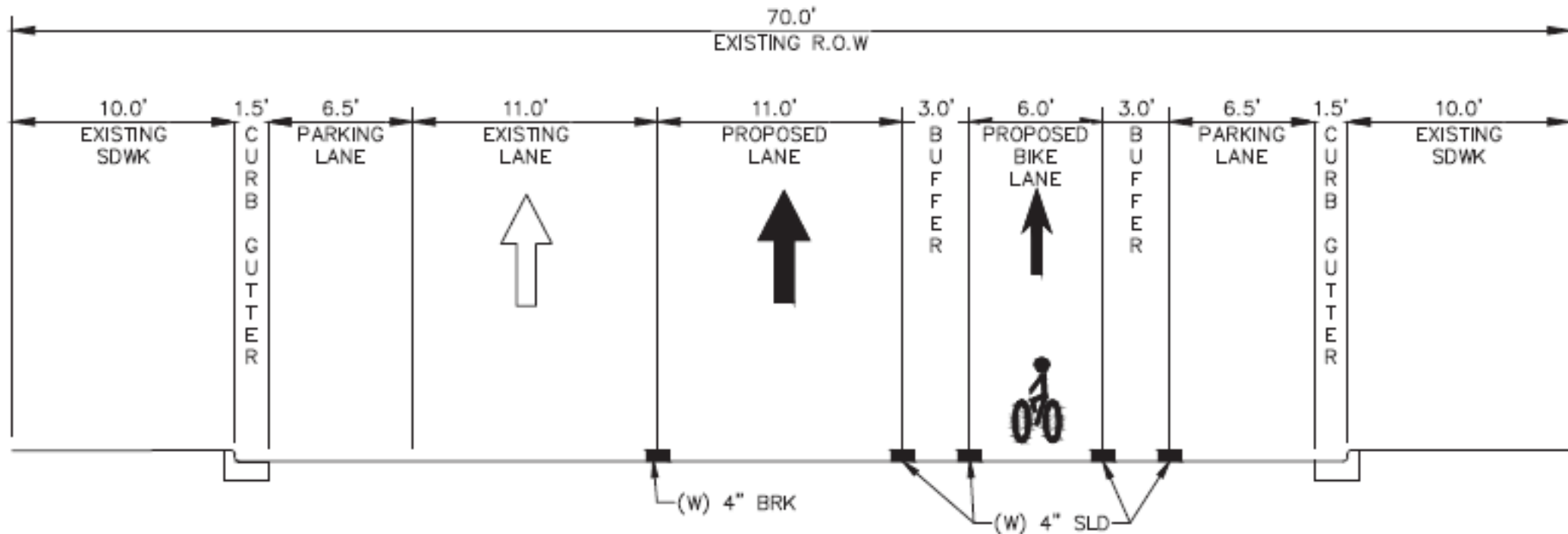
MISSOURI-KANSAS TO MESA PROPOSED TYPICAL SECTION
