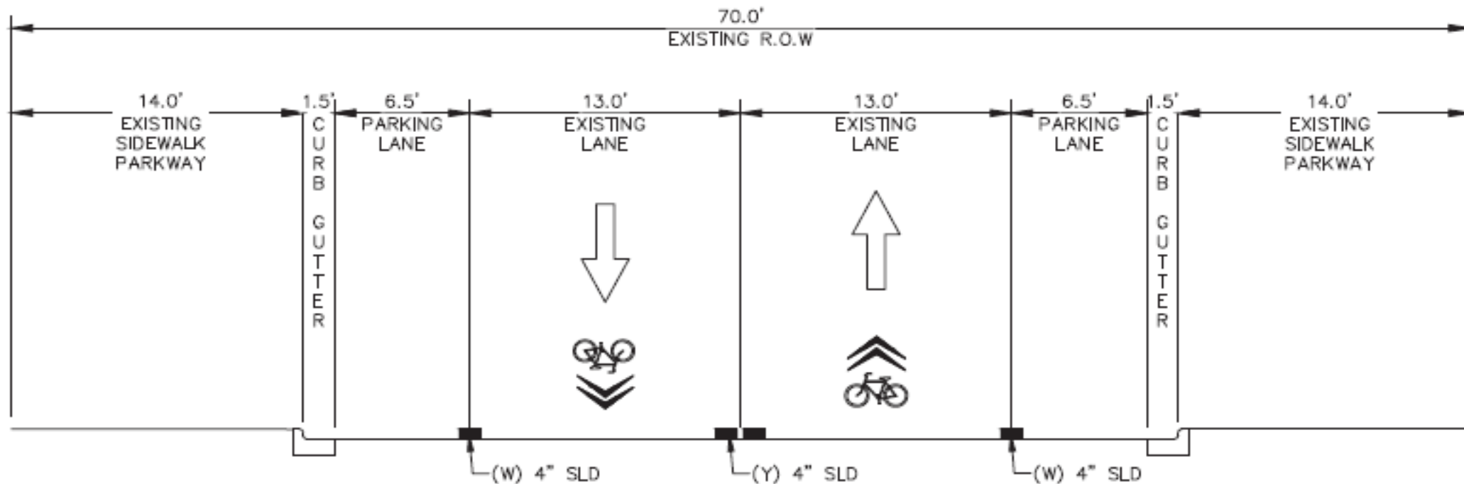
OVERLAND-EL PASO TO ST VRAIN PROPOSED TYPICAL SECTION
