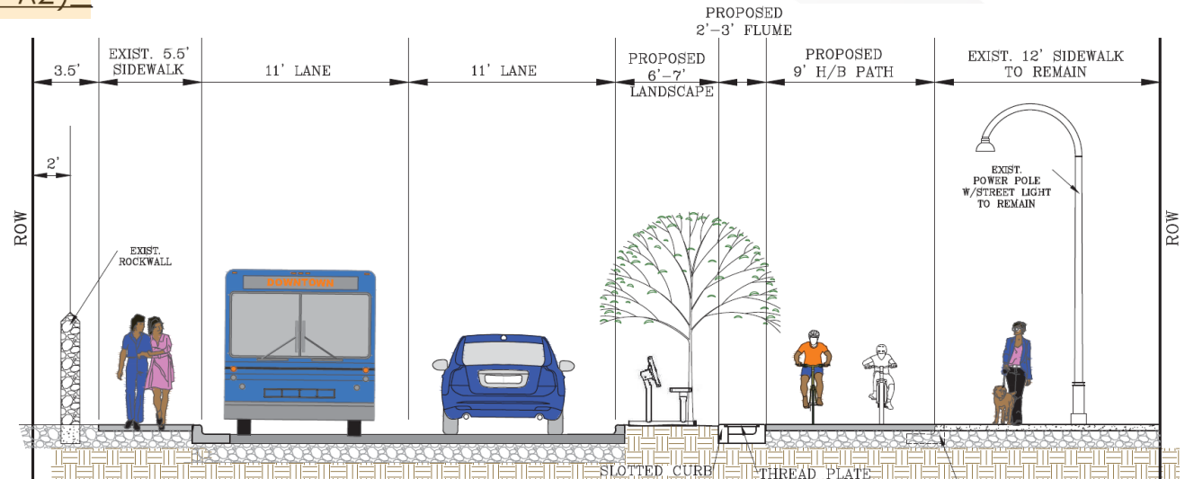
Parking Restricted (west side) 60' R.O.W. CROSS SECTION (B2 – B2) NTS
