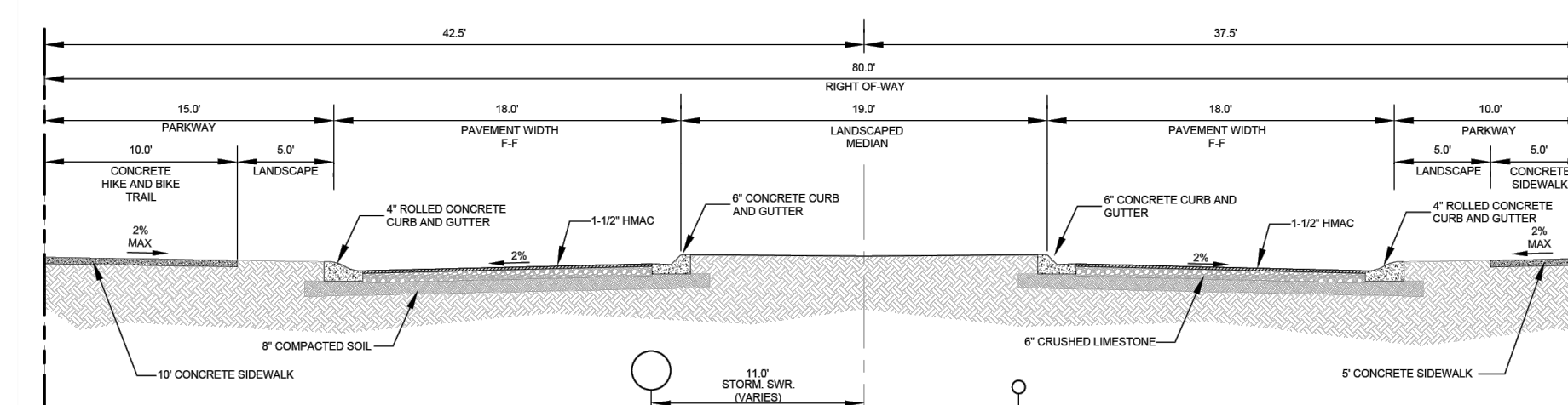
SECTION B-B 80' DIVIDED LOCAL STREET DESERT CALICO AVENUE WEST NTS
