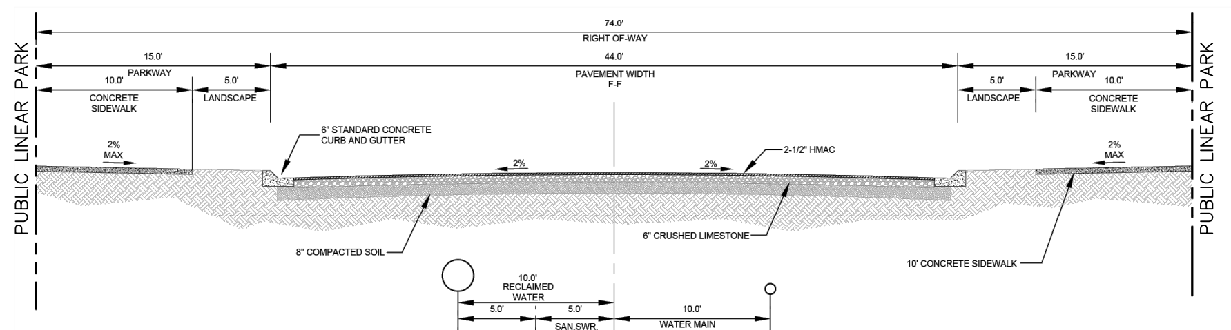
SECTION A-A 74' PRESTON FOSTER BLVD. RESIDENTIAL COLLECTOR STREET NTS
