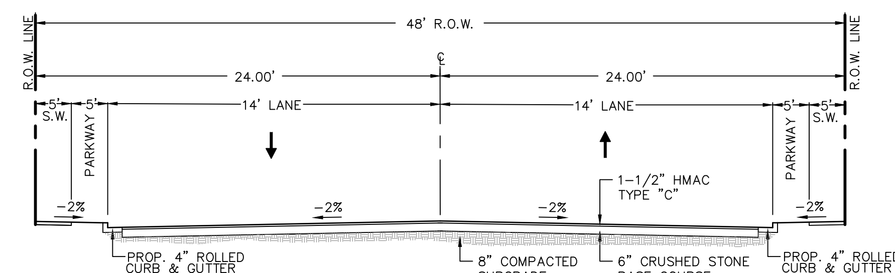
(PROPOSED) 48' R.O.W. TYPICAL SECTION ( LOCAL STREET )
