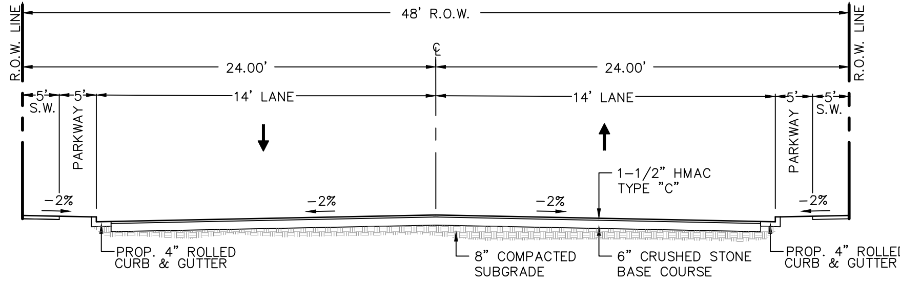
(PROPOSED) 48' R.O.W. TYPICAL SECTION (LOCAL STREET)
