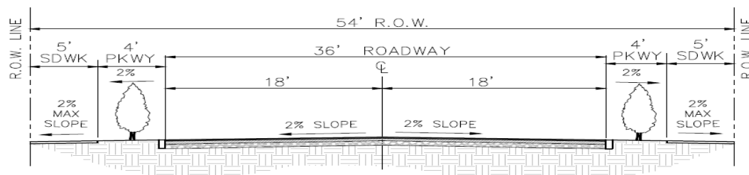
PROPOSED LOCAL RESIDENTIAL STREETS SECTION SECTION B-B SINGING RIVER WAY, SADDLE RIVER STREET, OLD RIVER WAY, WINDING RIVER AVE
