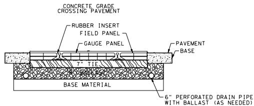
PROPOSED TYPICAL RAILROAD SECTION NTS
